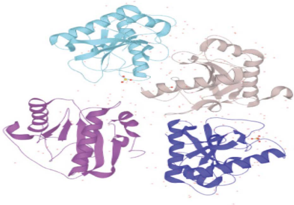
Fig. 1. Image showing the PDB structure of the protein as viewed under the UniProt.
